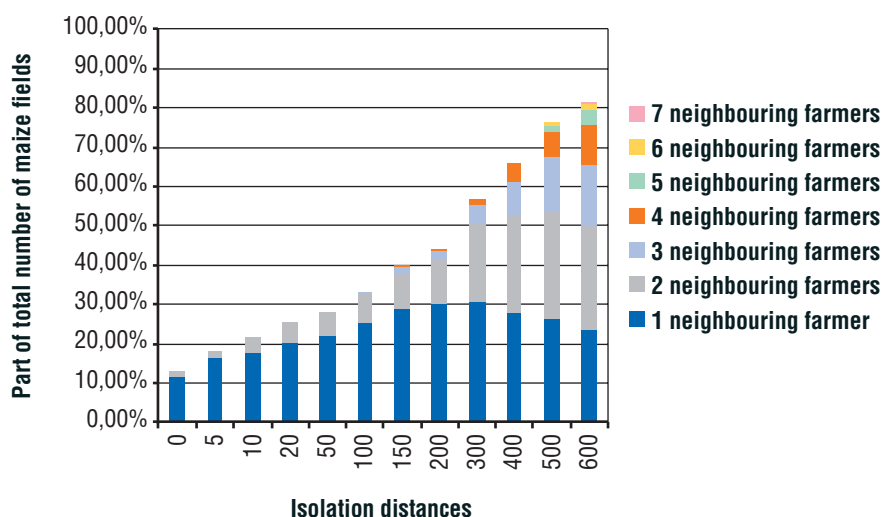
■ Figure 5: Maize fields (%) in the Poitou-Charentes region having neighbouring farmers owning maize fields within a given isolation distance
